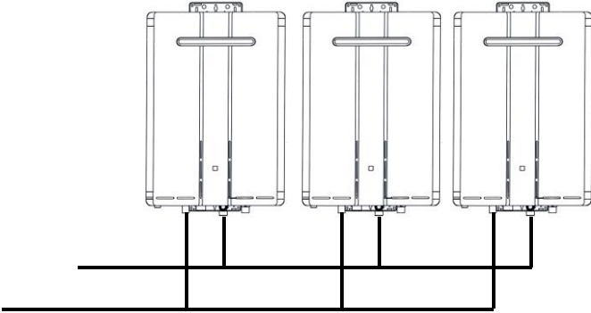
Unbalanced
