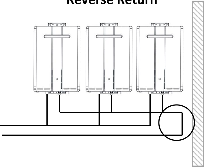
Reverse Return
